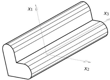
Fig. 2. Domain elongated along the axis x_3 with a constant cross section
