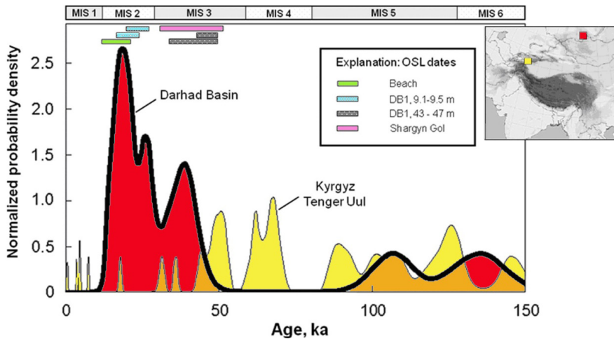
Fig. 11. Glacial chronology from Darhad Basin, southern Sayan range in Mongolia [12], and the Kyrgyz Tien Shan (Tenger Uul: 'Uul' = mountain range) [14]. The curves are for the ^{10}\text{Be} dates. Above the curves are rectangles giving the OSL dates for the glacial paleolake that filled Darhad Basin. In the explanation, 'DB1' refers to the Darhad Basin core extracted near the town of Renchinkhümbe in 2004; Shargyn Gol refers to a prominent cut bank through the lake sediments north of the drill site. Bars at the top show the marine oxygen isotope stages (MIS) defined by changes in \delta^{18}\text{O} in marine fossils. The chronology in Darhad Basin is essentially synchronous with the sea-level curve (fig. 3). The red square in the right center of the index map shows the location of Darhad Basin; yellow box in left center shows the Kyrgyz Tien Shan
