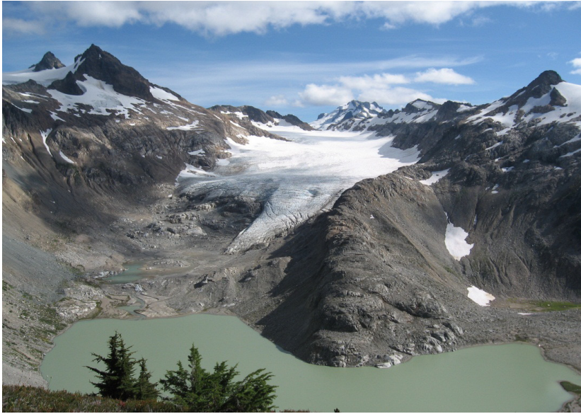
Fig. 1. Photograph of the South Cascade Glacier in retreat, Cascade Mountains. The landscape has been modified by repeated glaciation. The steep cliffs above the lateral margins of the glacier were produced by glacial erosion and mark the height of the glacier during the Ice Age. Ablation zone is the darker part of the glacier near its terminus, where light-toned snow has melted. View to SE. Photograph: Kurt Parker, 2007
